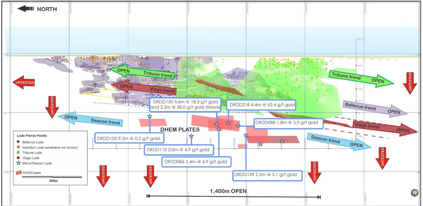
Figure 1: Long section looking east of the Bellevue Lode system. The new Deacon & Mavis discovery is located immediately below and offset 400m to the east of the Bellevue Mine.
