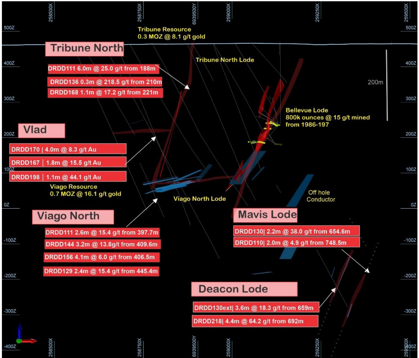
Figure 3: Cross Section through the Bellevue Lode system looking North showing the location of the new Deacon and Mavis Lodes located 400m into the footwall of the Bellevue Lode 1
